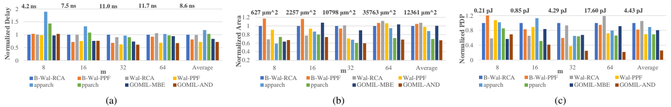
Fig. 3. Delays, areas, and power-delay products of the existing and the proposed multipliers for different word lengths. The values of B-WAL-RCA are listed above each group.
