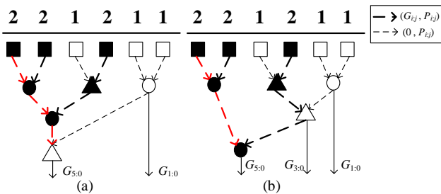
Fig. 2. Two prefix trees for the same input BCV.
